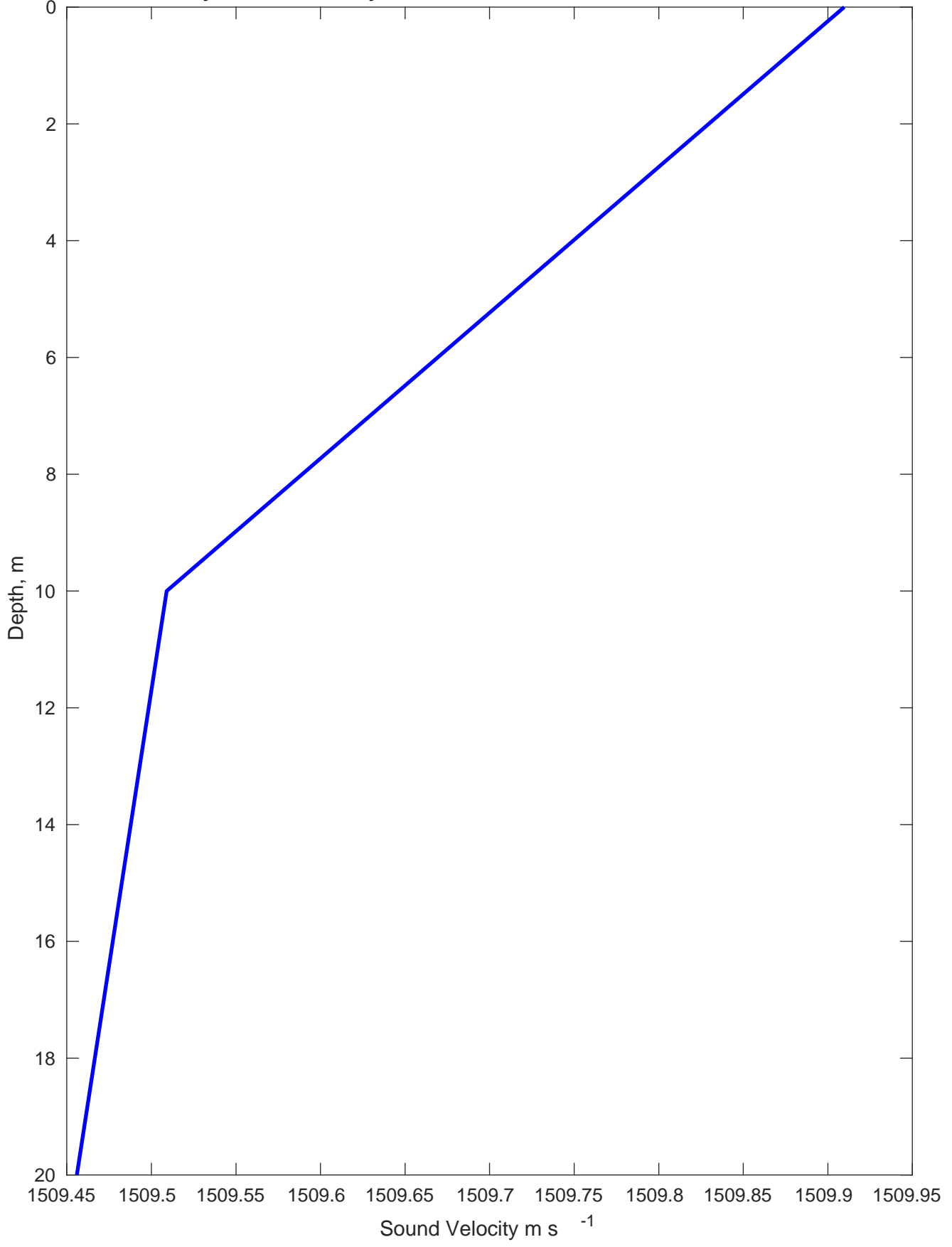
Sound Velocity Profile for Vineyard Wind GB22 on 13-Oct-2022 00:00:00
